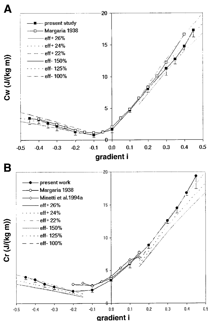
Fig. 1. Metabolic energy cost of walking (Cw; A) or running (Cr; B) as a function of the gradient from the present investigation and from the work by Margaria (14, 15) and Minetti et al. (20, only for running). Minimum energy cost of walking and average energy cost of running for each gradient have been reported. To accurately describe the relationship between Cw or Cr and the gradient i within the investigated range, 5th-order polynomial regressions were performed, that yielded
