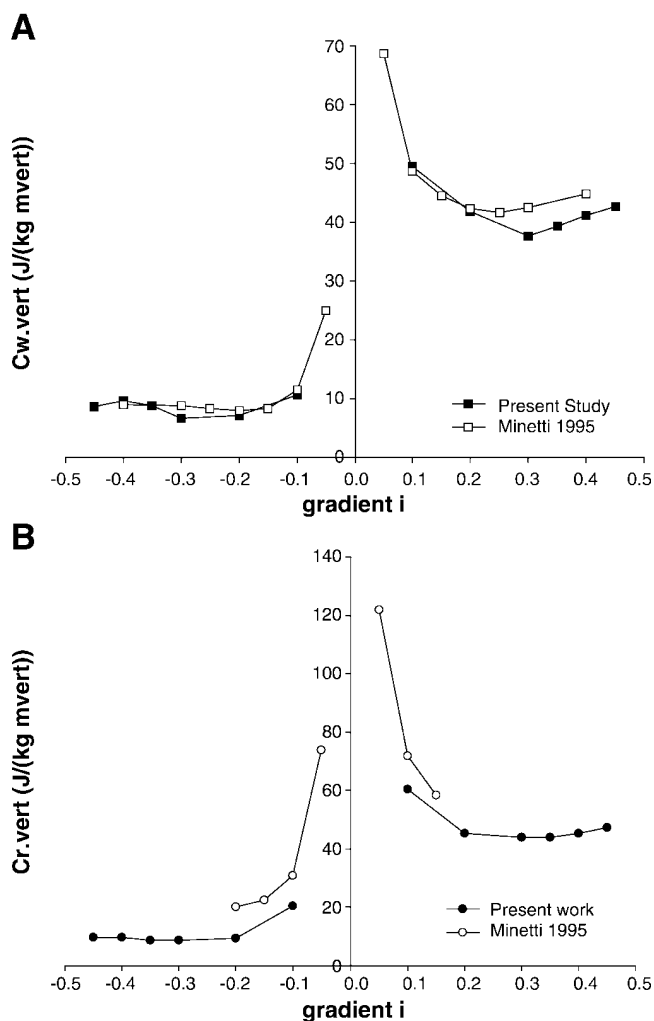
Fig. 2. Metabolic energy cost of walking (A) or running (B), expressed per unit of vertical distance ( m_{\text{vert}} ) as a function of the gradient, from the present investigation ( \blacksquare ), and from Minetti (18), where reprocessed data from Margaria (14, 15) were presented.
