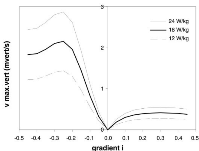
Fig. 5. Maximum running speed, expressed in vertical meters per second, vs. gradient, as predicted by combining Eqs. 2 and 3. The three curves refer to different \dot{V}O_{2 \text{ submax}} values (net metabolic powers of 12, 18, and 24 W/kg).
